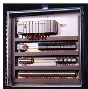
Low-voltage control center separate from high-voltage on high horsepower machines.
